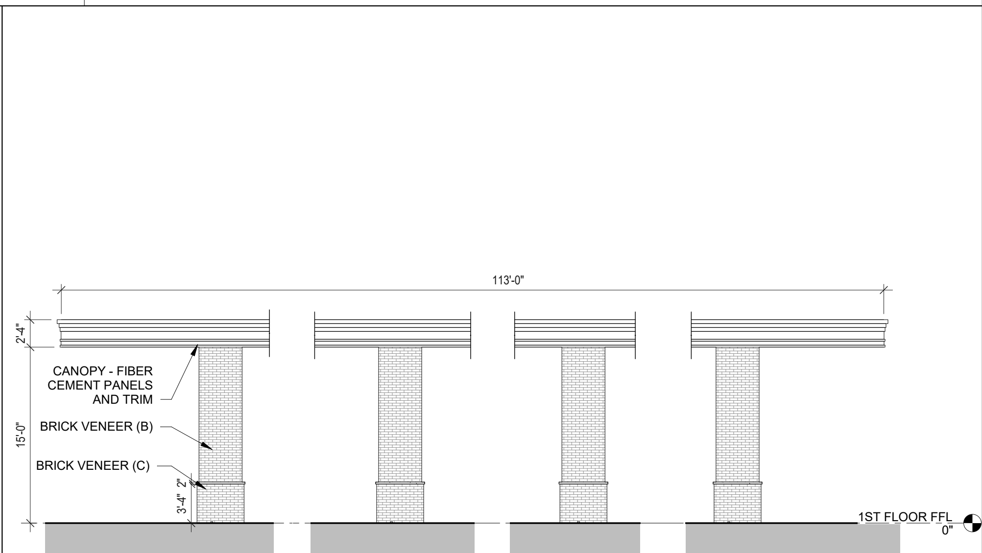
D5 EXTERIOR ELEVATION - EAST CANOPY 1/8" = 1'-0"
